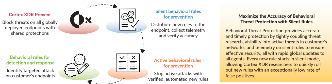
Figure 2: Behavioral Threat Protection with Cortex XDR
