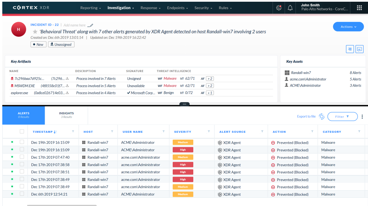
Figure 5: Investigate and respond to attacks
